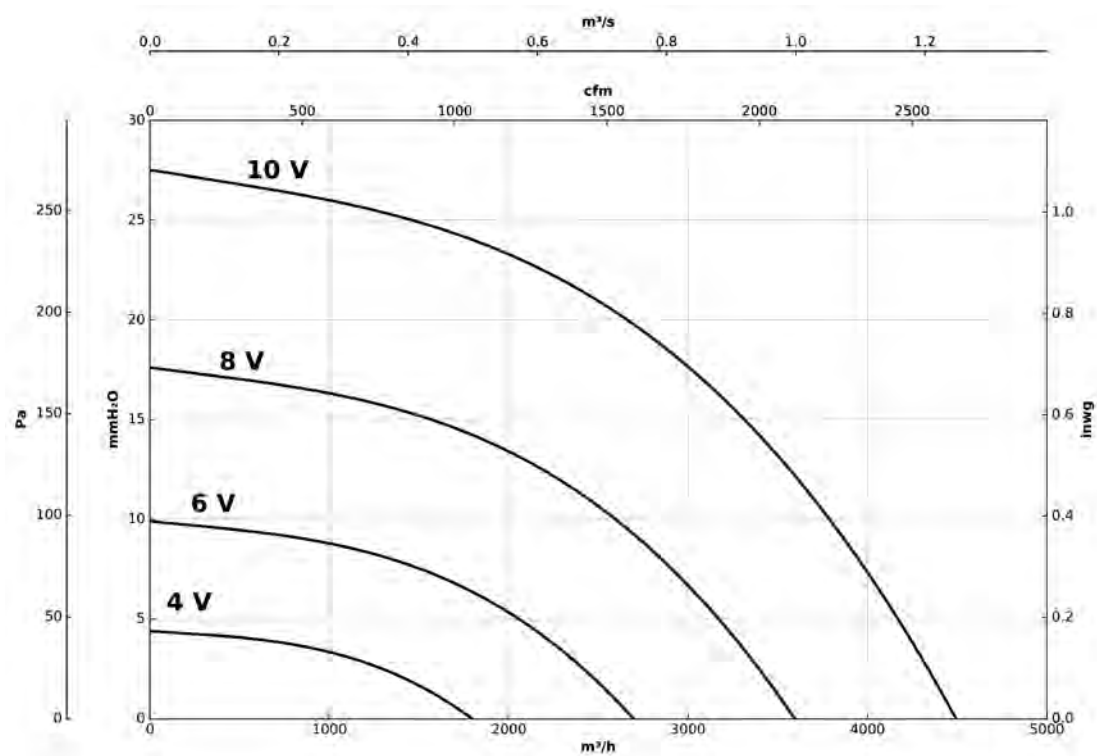
CHT/EC-400-6M
