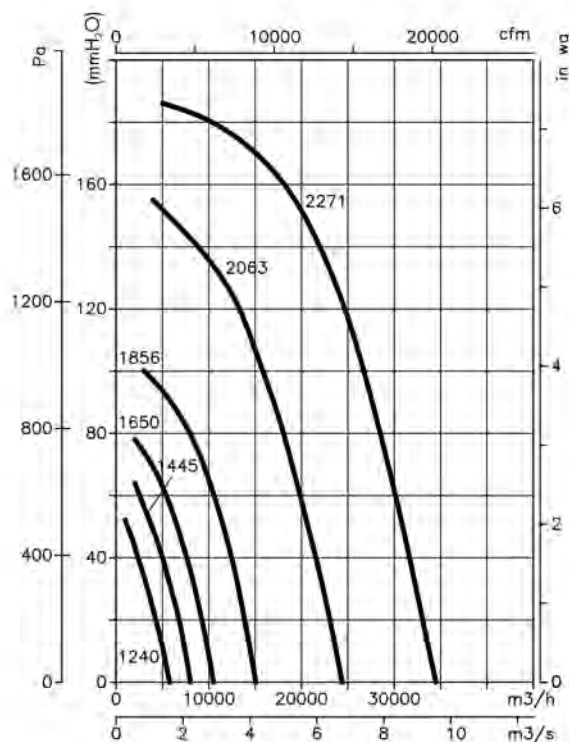
4T=1500 r/min
