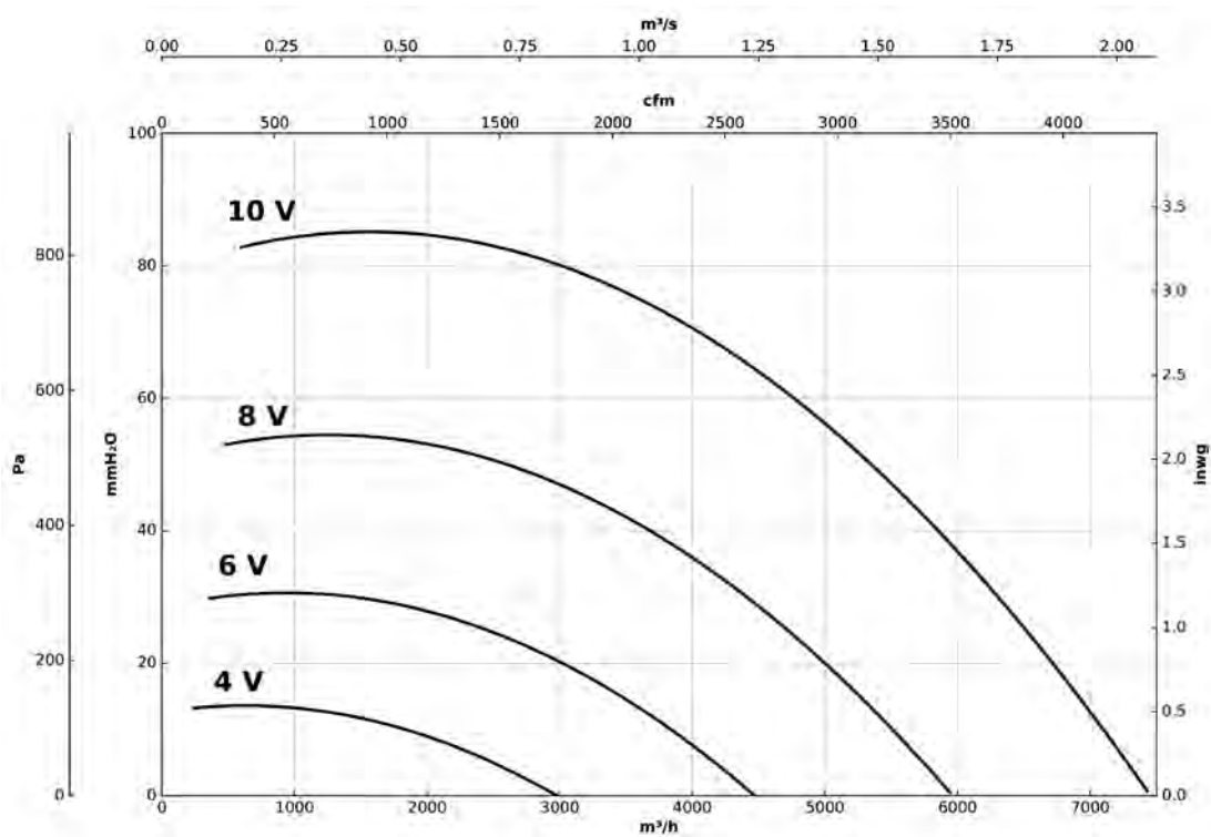
CKDR-500-4M-1.5 IE5
