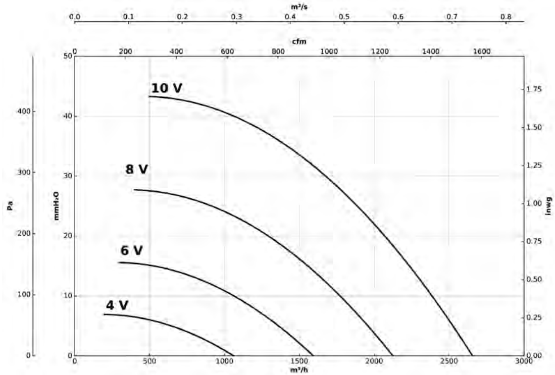
CKDR-355-4M-0.5 IE5
