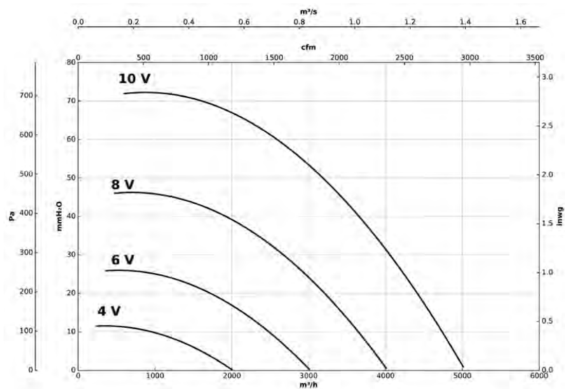
CKDR-450-4M-1 IE5
