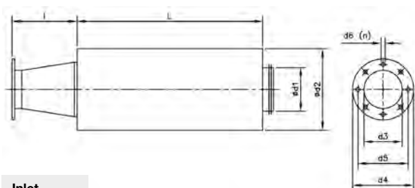
Inlet
