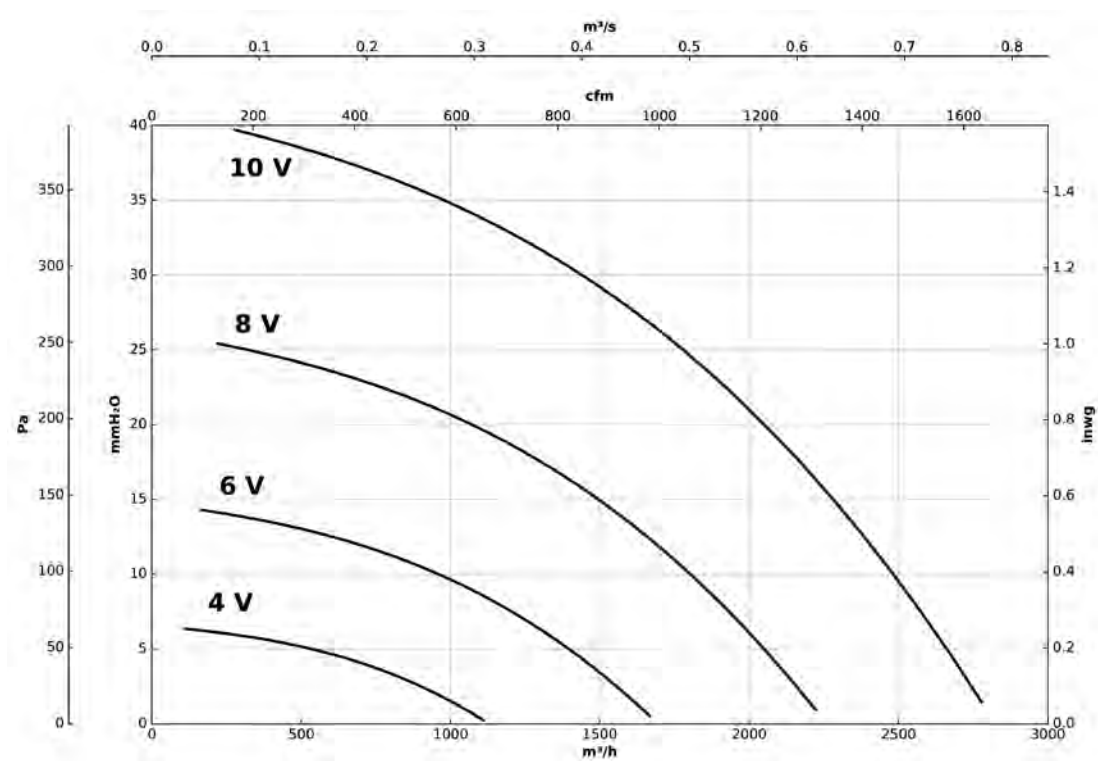
CJLINE/EC-1235-4M
