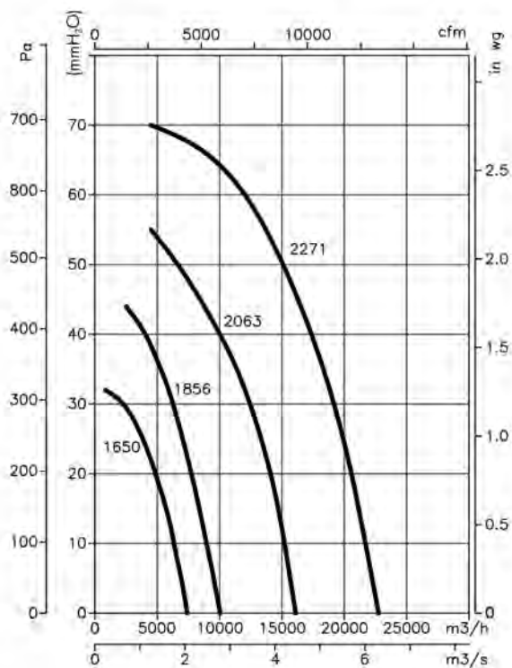
6T=1000 r/min
