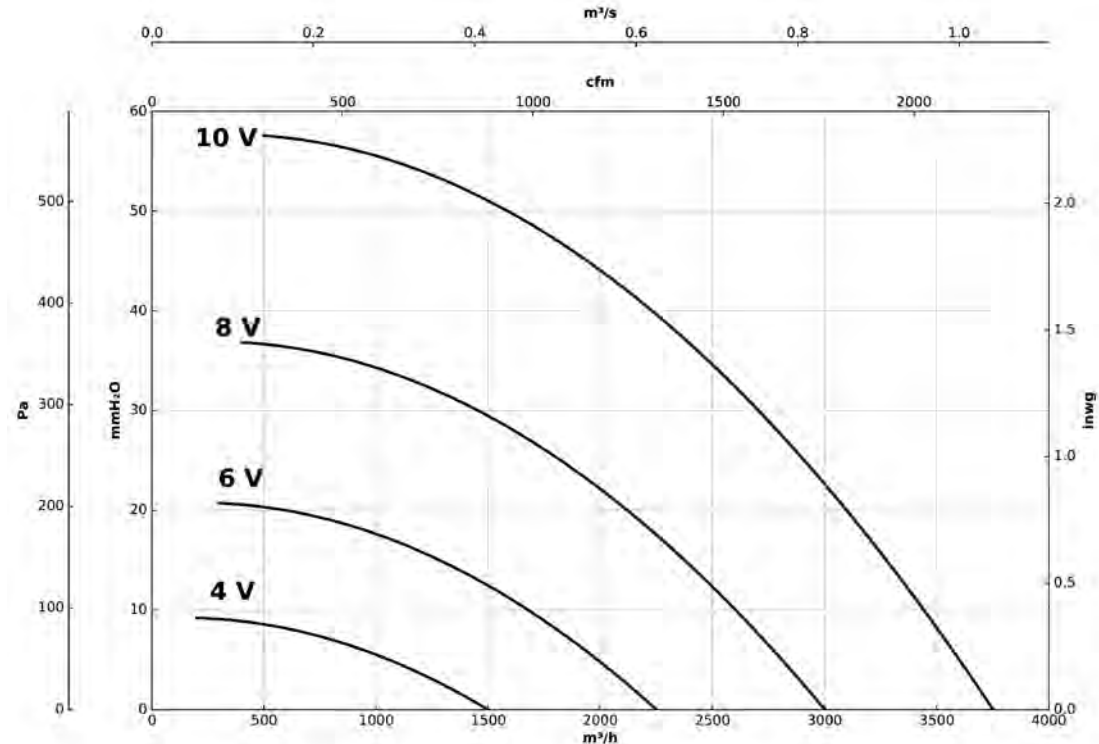
CKDR-400-4M-0.75 IE5
